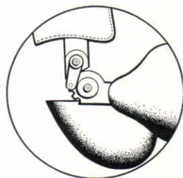
Fig. 12. Robin-Aids stump-actuated elbow lock.
