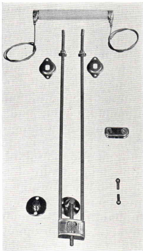
Fig. 17. Twin-cable control system for below-elbow biceps cineplasty.
