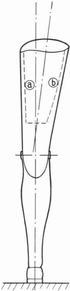
Fig. 5. Posterior view of the above-knee prosthesis showing position of the socket in relation to the rest of the leg. The medial line (a) should be approximately vertical. The lateral line (b) is sloped downward and inward. From Had-dan (8).
