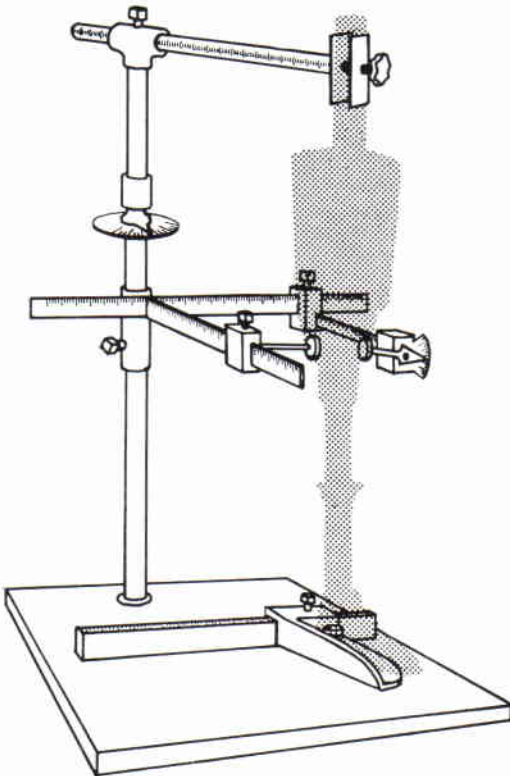
Fig. 8. Schneider's alignment stand.
