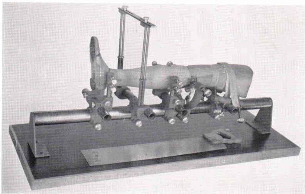
Fig. 12. The alignment duplication jig.
