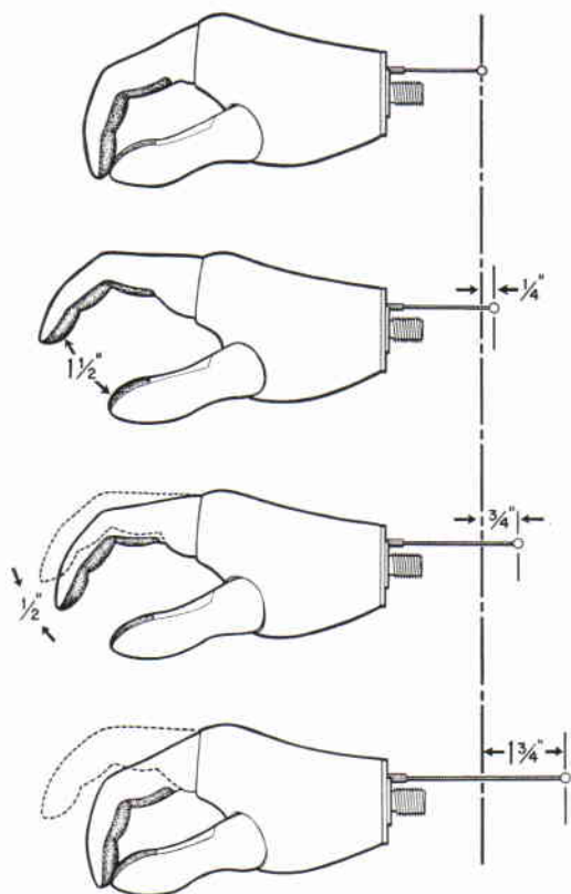
Fig. 14. The principle of the reflex hand. First \frac{1}{4} in. of excursion in the control cable opens the hand to the full 1\frac{1}{2} in. Further pull on the cable closes the hand at a 1:1 ratio of finger-tip travel to cable travel. Thus, after 1\frac{3}{4} in. of cable travel, the hand is fully closed again. The difference between the 1\frac{3}{4} in. total excursion and the ideal 1\frac{1}{2} in. may be compensated for during the closing cycle by lineating mechanisms which give \frac{1}{4} in. actual cable travel. Upon release of tension on the cable, the action goes through the reverse cycle. The hand first opens fully (at a ratio of 1:1). Last \frac{1}{4} in. of cable excursion allows hand to return to closed or "rest" position. The excursion relationships suggested here are approximations; they may need minor modification on the basis of actual experience with test wearers.
