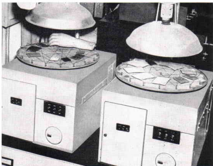
Fig. 5. Apparatus, consisting of ultraviolet lamp and turntable, for determining color fastness of pigments and degradation of plastic materials under exposure to simulated sunlight. Courtesy Army Prosthetics Research Laboratory.
