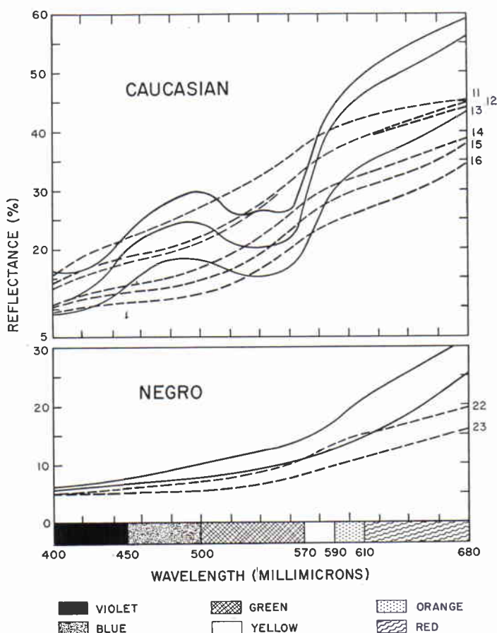
Fig. 3. Spectrophotometric curves for the dorsal skin of Caucasian and Negro hands and for Caucasian and Negro cosmetic gloves. Above, curves for Caucasian hands (solid lines, three subjects) and for cosmetic gloves, shades 11 through 16 (dashed lines). Below, curves for Negro hands (solid lines, two subjects) and for shades 22 and 23 of the Negro glove (dashed lines).
