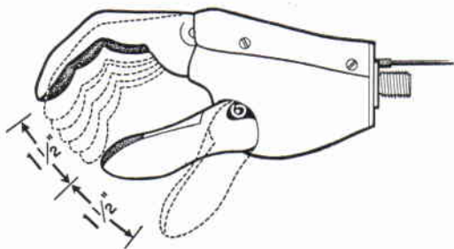
Fig. 11. The two-position thumb, set manually from either position to the other by application of pressure on the dorsal side. Inner position provides for objects up to 1\frac{1}{2} in. Outer position accommodates objects between 1\frac{1}{2} and 3 in.
