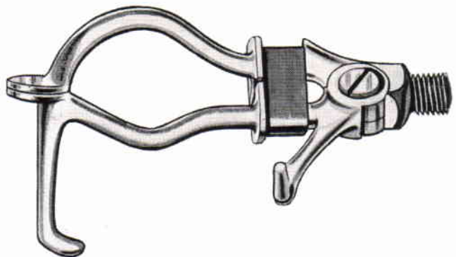
Fig. 7. The Dorrance No. 3 hook, a voluntary-opening terminal device of highly specialized design sometimes used by farmers, laborers, mechanics, and others engaged in various kinds of manual work.
