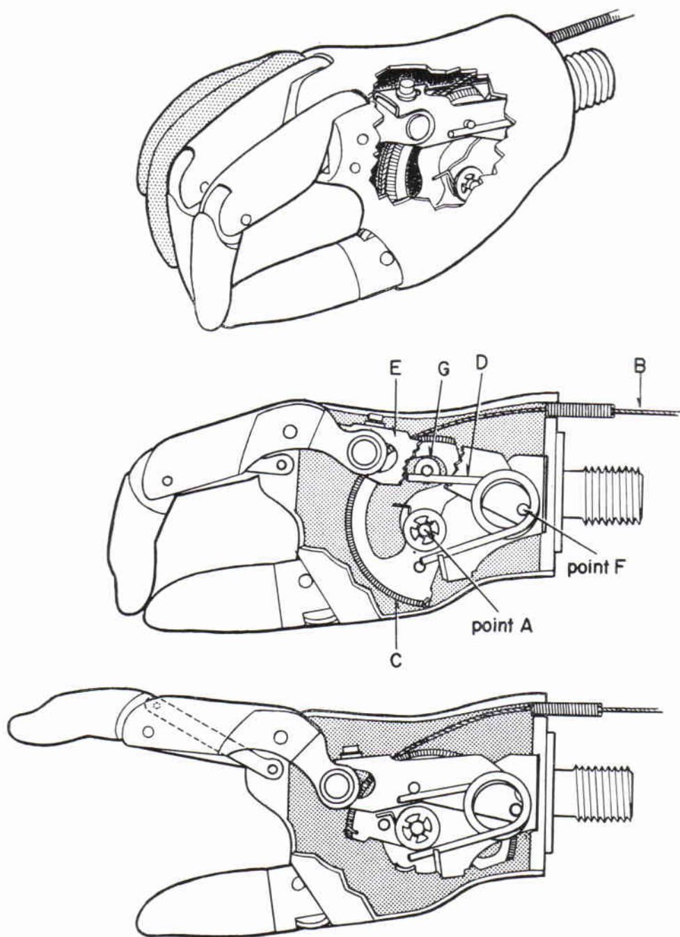
Fig. 3. Cutaway views of the APRL-Sierra Model No. 1 Hand (3). When no tension is applied to the control cable B , spring D forces the index and middle fingers toward the thumb to provide prehension of the three-jaw-chuck type. Tension in the control cable B causes the quadrant C to rotate about point A , a point displaced from the true center of quadrant C . The cam action thus provided by the outer edge of the slot in quadrant C against roller G forces lever E to rotate counterclockwise about point F , in turn causing the index and middle fingers to open. A small brass plate is mounted within lever E in such a fashion that, when little or no tension is applied to the control cable, the plate wedges against the periphery of the quadrant C . The wedging action, known as "Bac-Loc," resists opening of the fingers when force is introduced through the finger linkage but has no effect on the system when force is applied through the control cable.
