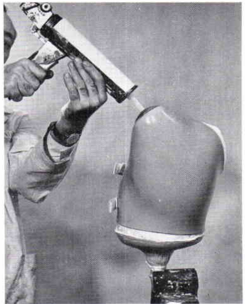
Fig. 21. Injection of silicone foam through center hole of spherical plate.
