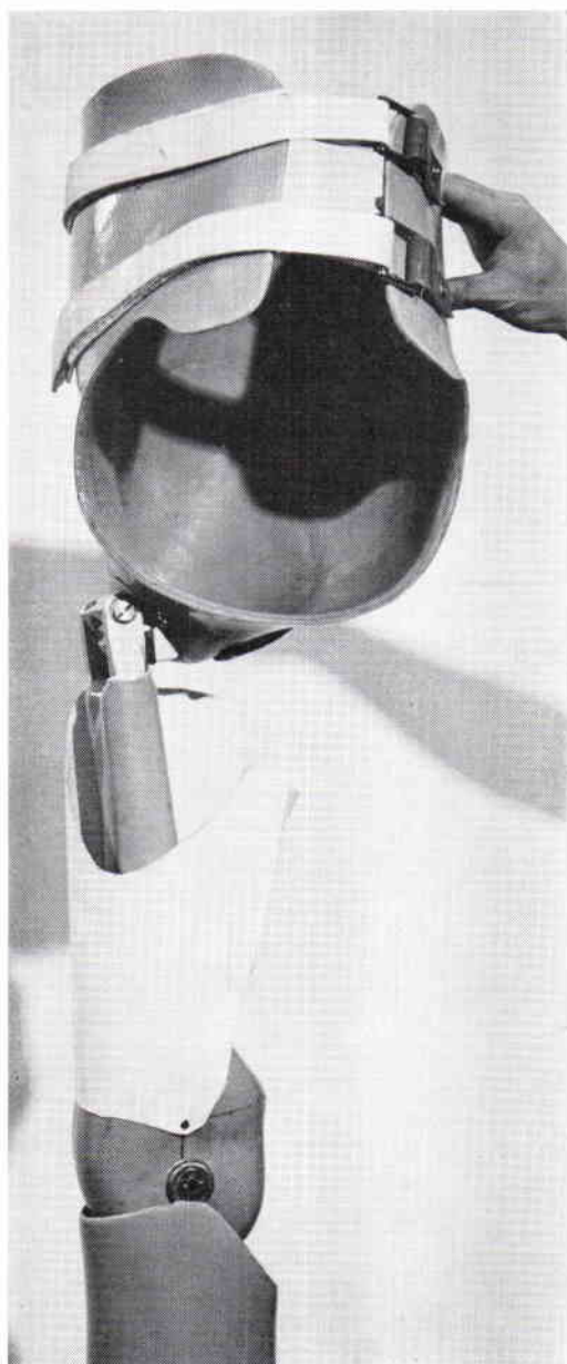
Fig. 29. Cardboard used as template for metal portion of thigh fairing.
